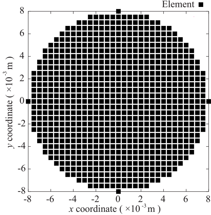
Figure 4.6: Element pattern for a 797-element array.
