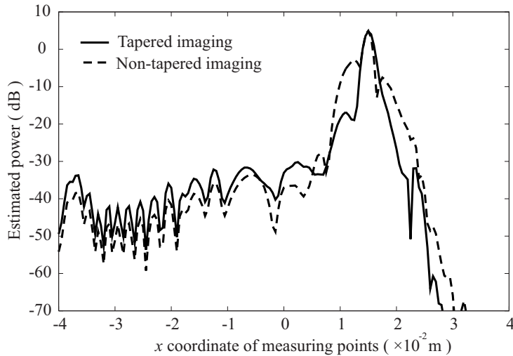
Figure 4.14: Lateral resolution of a tapered and non-tapered proposed imager with a 0.016 m width array in a 3-D problem. The x coordinate of a target is 0.015 m, and those of the measuring points are -0.04 to 0.04 m.
