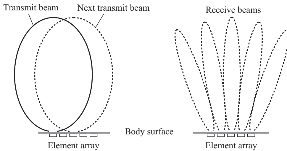
Figure 1.16: Transmit and receive schemes of a synthetic aperture imager. A wide transmit beam is radiated to the entire measurement plane. Then all the image lines in the measurement plane is formed in parallel. In the next transmit event, a transmit beam is radiated from the next transmit point.
