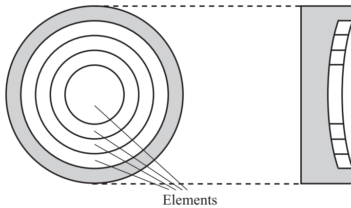
Figure 1.8: Schematic view of an annular array probe.
