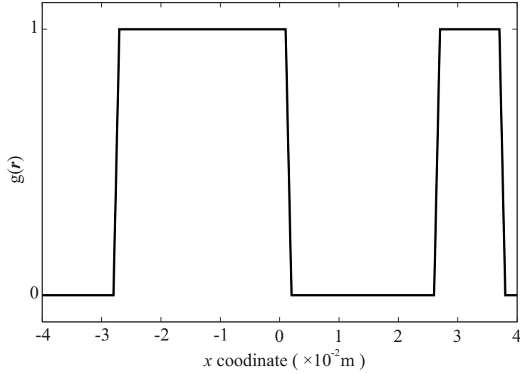
Figure 4.8: The area used on the mirror in the x-z section. The value of used area is 1 and that of non-used area is 0. The x, y and z coordinates of a target are 0.005, 0 and 0.07 m respectively.
