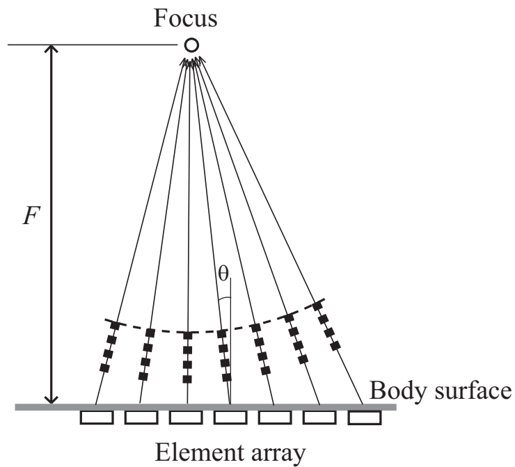
Figure 1.11: Schematic view of the beam formation employed by a sector scan probe.
