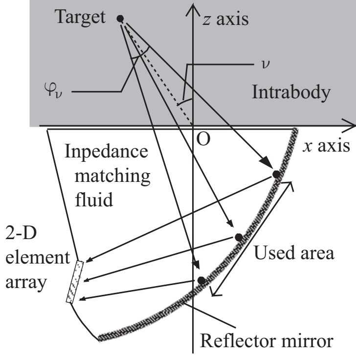
Figure 4.2: Schematic view of the system in the receive phase.
