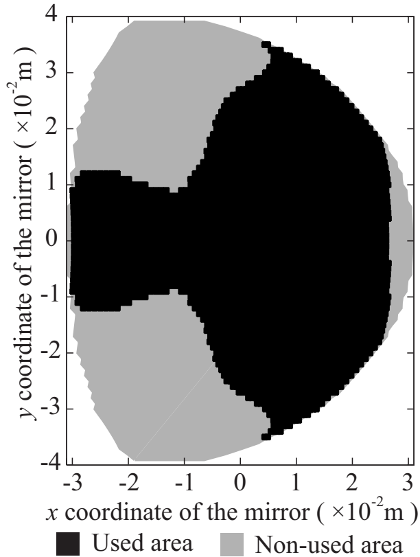
Figure 4.11: The used area on a mirror projected onto the x-y plane where a target exists at the center for a 0.07 m depth.
