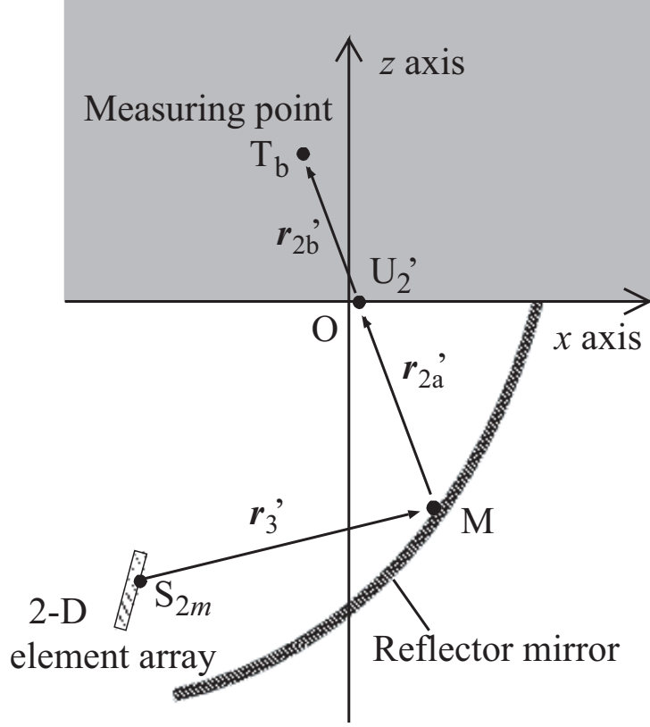
Figure 4.5: Arrangement of a 2-D element array and a mirror in the receive phase.
