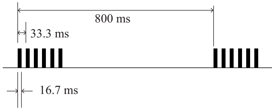
Figure 5.10: Stimulus waveform in the simultaneous stimulation trials. Pulse repetition rate is 30 Hz and pulse width is half of the pulse onset interval. Each burst has 6 pulses and burst onset interval is 800 ms.
