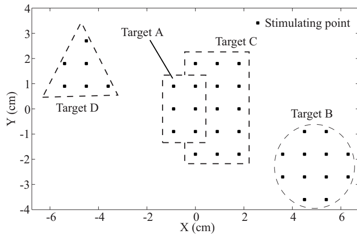
Figure 5.6: Stimulating points matched with targets when the measurement range is d_2 .
