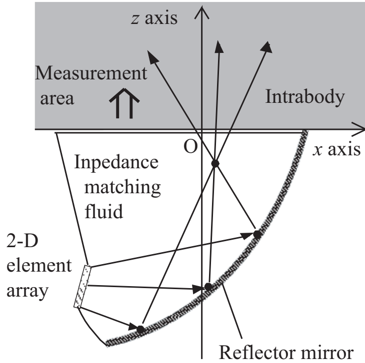
Figure 4.1: Schematic view of the system in the transmit phase.
