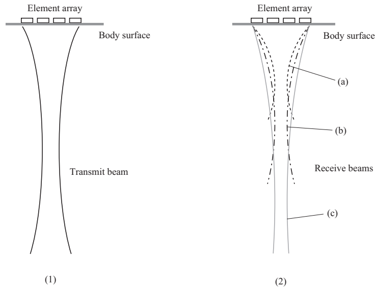
Figure 1.13: Schematic view of the dynamic beam focusing. (1) Single transmit beam is radiated for one measurement direction. (2) In the receive phase, the element array employs various sets of time delays to acquire a narrow receive beam at each measurement range. The receive beams (a), (b), and (c) are formed for short, middle, and long range measurement, respectively.
