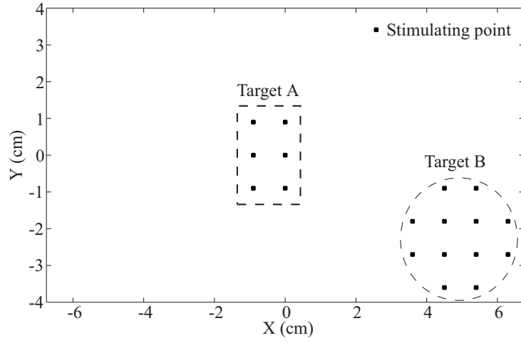
Figure 5.5: Stimulating points matched with targets when the measuring range is d_1 .
