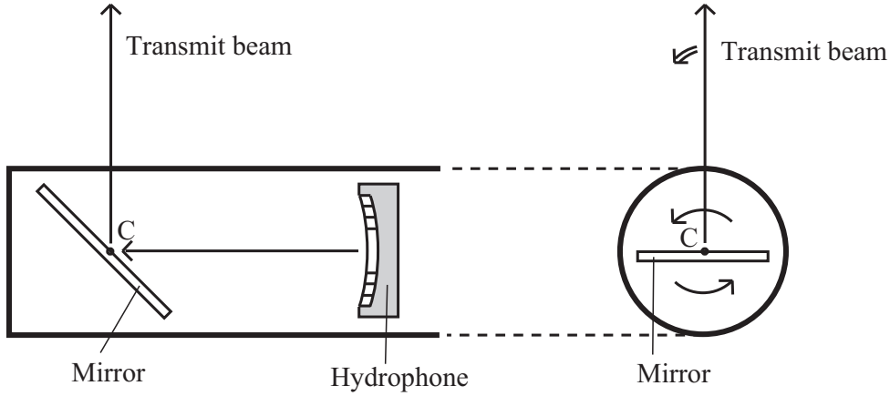
Figure 1.9: Schematic view of an endoscope with a radial scan imager. The left and right figure is the longitudinal and cross section of the endoscope.
