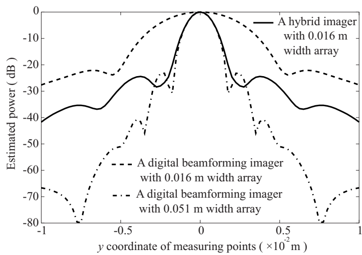
Figure 4.19: Lateral resolution of the proposed imager with a 0.016 m width array and digital beamforming imagers with 0.016 m and 0.051 m width arrays. A target exists at the center for a 0.07 m depth.
