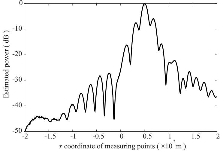
Figure 4.9: Lateral resolution where the used area consists of plural groups. The main lobe divides, and thus the sidelobe level becomes high.
