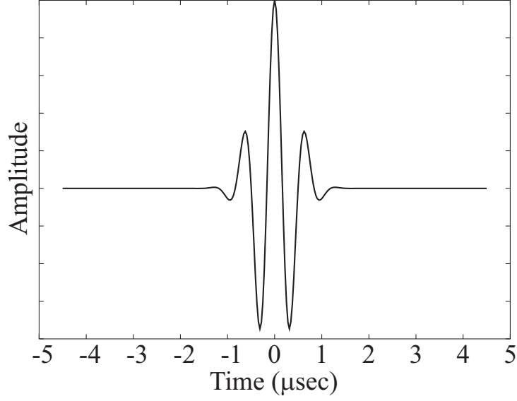
Figure 4.7: Waveform of the pulse used in this paper.
