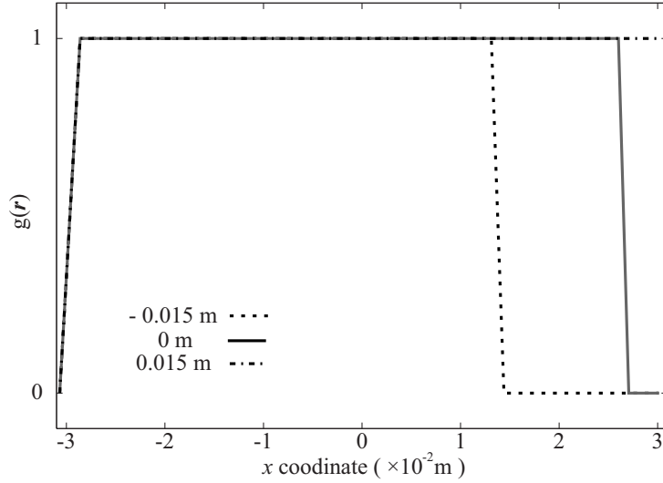
Figure 4.10: The used area on the optimized mirror in the x-z section. The value of the used area is 1 and that of the non-used area is 0. The x coordinates of targets are -0.015 , 0 and 0.015 m. The target range is 0.07 m in the x-z section.
