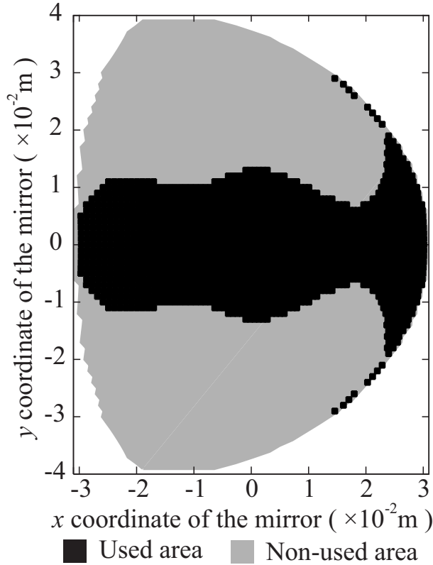
Figure 4.12: The used area on a mirror projected onto the x-y plane where the x coordinate of a target is 0.015 m in the x-z section for a 0.07 m depth.
