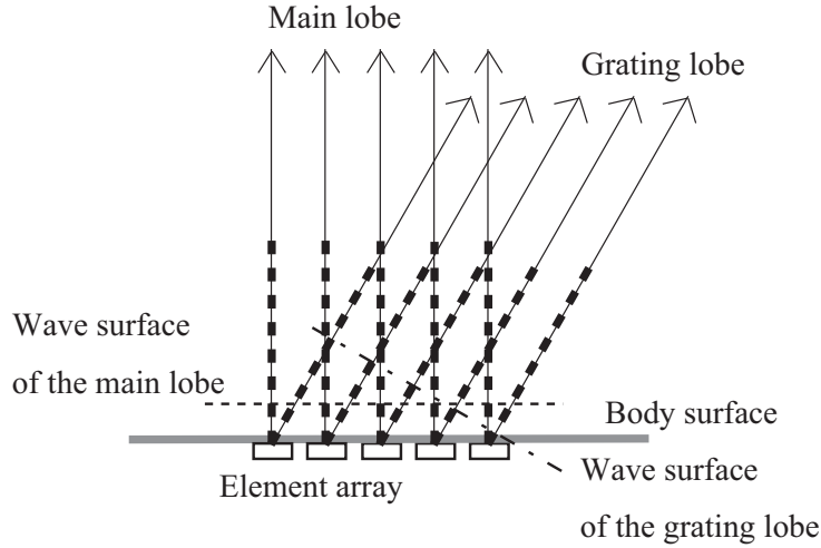
Figure 1.12: Grating lobe appeared in the measurement field. An unwanted lobe appears in a certain condition about element interval.
