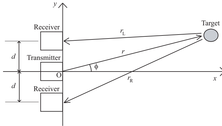
Figure 1.5: Schematic view of the detection of target direction with two receive elements.
