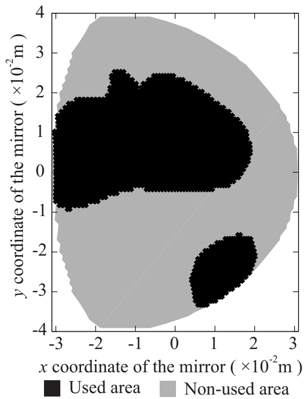
Figure 4.18: The used area on a mirror projected onto the x-y plane where the y coordinate of a target is 0.015 m in the y-z section for a 0.07 m depth.
