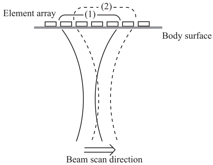
Figure 1.10: Beam scanning from the change of actibated elements. The change of actibated elements from (1) to (2) causes the beam scan to the right direction.
