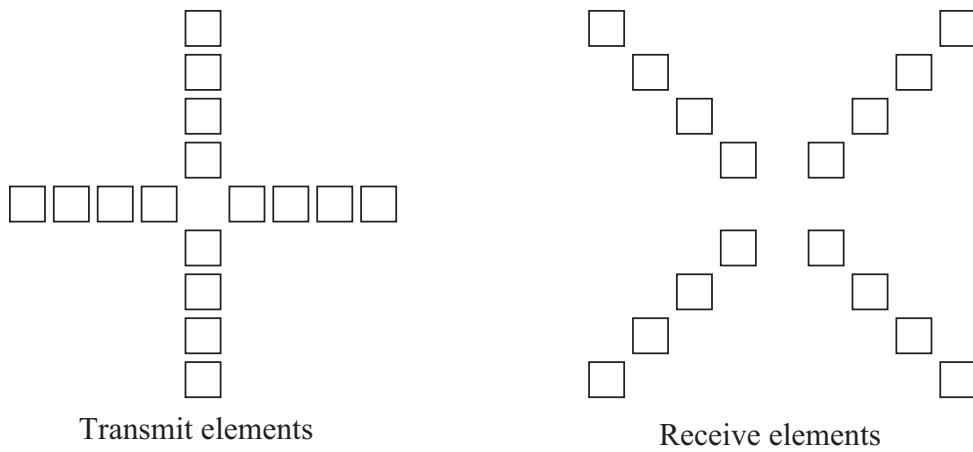
Figure 1.19: A 2-D element array design using different transmit and receive geometries. Since a transmit beam and a receive beam have different radiation patterns, the directions of grating lobes are different by each other. Therefore grating lobes are suppressed.
