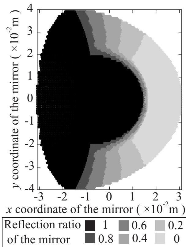
Figure 4.13: The taper function for the reflection ratio on the mirror in numerical back projection.
