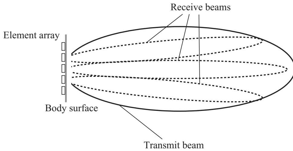
Figure 1.15: Schematic view of multi-line imaging.
