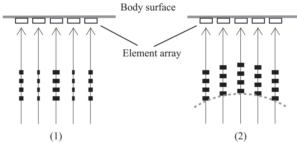
Figure 1.18: Transmit schemes using multiple elements to synthesize a single element response. Multiple elements are excited (1) simultaneously with apodization, and (2) with a set of time delays to form defocused ultrasound pulses.
