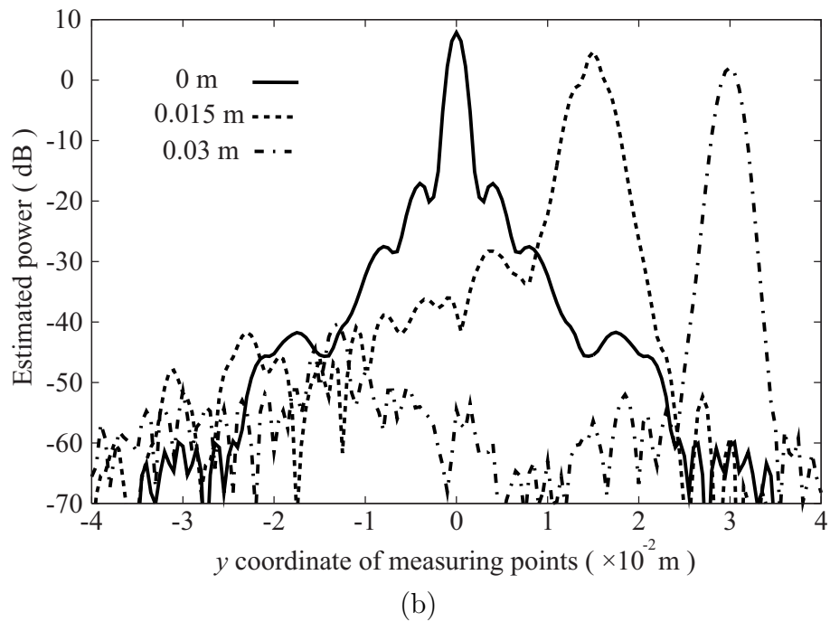
Figure 4.17: Lateral resolution of the proposed imager with a 0.016 m width array in the (a) x-z and (b) y-z sections for a 0.07 m depth. (a) X coordinates of targets are -0.03, -0.015, 0, 0.015 and 0.03 m. (b) Y coordinates of targets are 0, 0.015 and 0.03 m.
