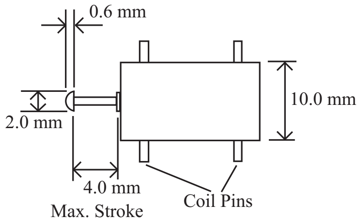
Figure 5.9: Schema of a solenoid component in the 2-D stimulator array placed on the forehead.
