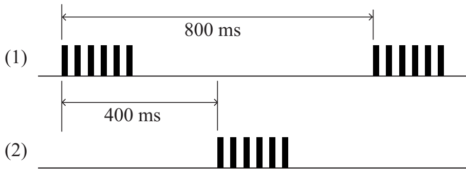
Figure 5.12: Stimulus waveform in the alternating stimulation trials. Waveforms (1) and (2) are delivered to the active solenoids of groups 1 and 2, respectively. Stimulus onset asynchrony between the two groups is 400ms.
