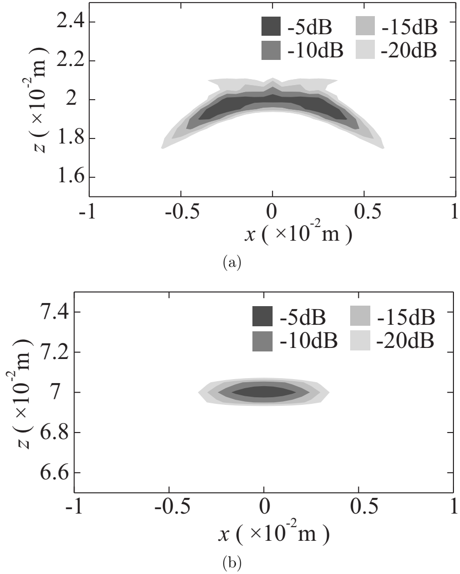
Figure 4.15: Spatial resolution of a phased array imager with a 1-D array. The focal length of the acoustic lenses is 0.07 m, and the targets exist at the center for depths of (a) 0.02 m and (b) 0.07 m. This section is perpendicular to the longitudinal axis of the linear array.
