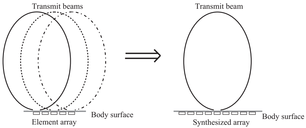
Figure 1.17: The effective aperture of the imager synthesized from multiple transmit and receive event. The coherent integration utilizing the synthetic aperture technique realizes a spatial resolution equivalent to that of an aperture given by the convolution of the transmit points and the receive aperture.
