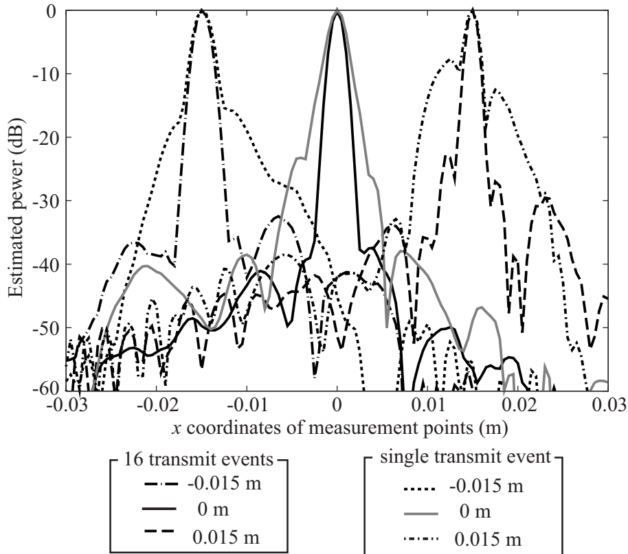
Figure 6.9: Lateral resolution of the proposed imager acquired from single and 16 transmit and receive events in the x - z section for a 0.07 m depth. The x coordinates of point targets are -0.015 , 0 and 0.015 m.
