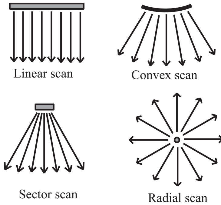
Figure 1.7: Schematic view of the scan types of B-mode imagers.
