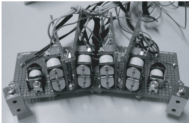
Figure 5.7: Solenoid array placed on participants' foreheads. The 2 \times 4 solenoids placed at the center of the array are the stimulators. The two solenoids placed at the sides always generate sound and vibration to prevent participants from distinguishing tactile patterns by sound.
