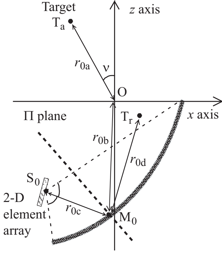
Figure 4.4: Schematic view of the mirror and array configuration for calculating in the time domain.
