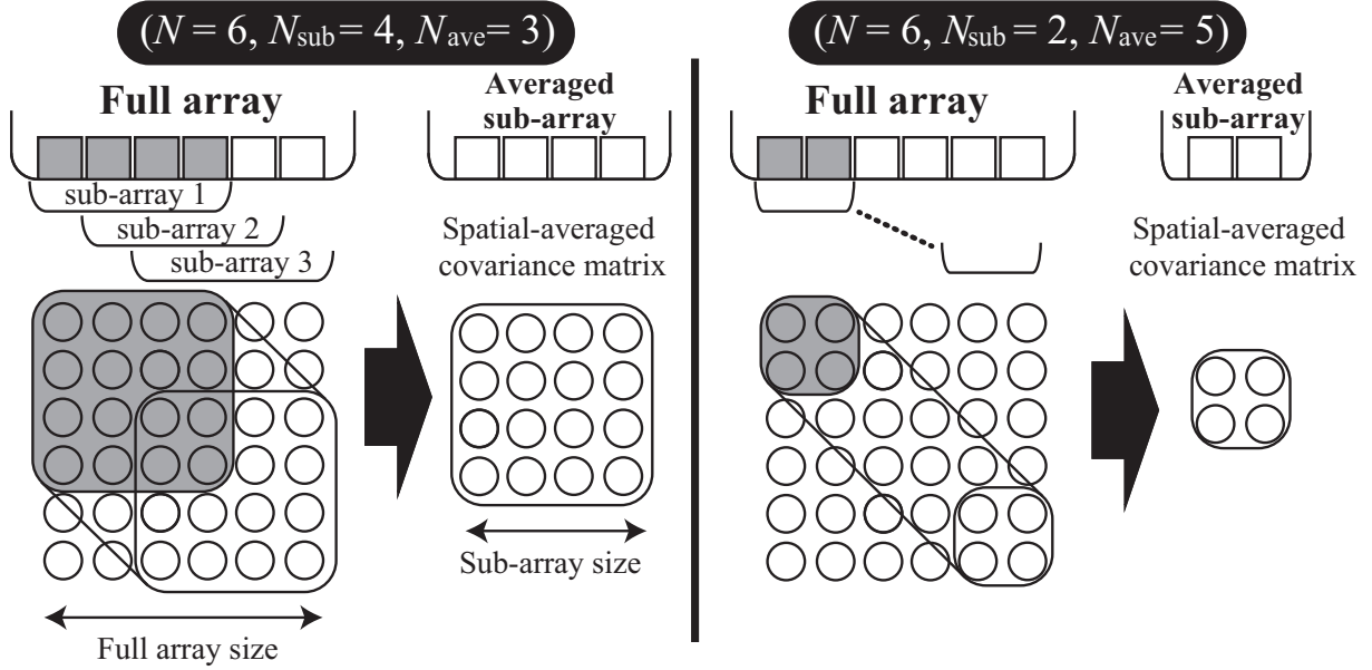
Figure 1.18: Schematic illustration of the sub-array averaging technique with two examples. (N, N_{\text{sub}}, N_{\text{ave}}) = (6, 4, 3) and (N, N_{\text{sub}}, N_{\text{ave}}) = (6, 2, 5) .
