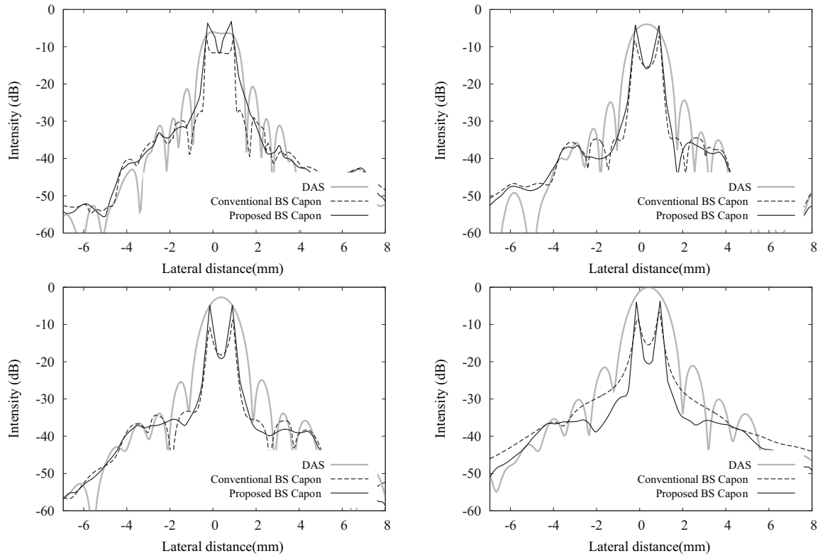
Figure 2.6: Experimental result of cross-sectional images at the target depth obtained by the DAS method, the conventional BS Capon, and the proposed BS Capon method. The lateral interval of the targets was 1.0 mm and the target depths were (a) 21.4, (b) 31.4, (c) 41.4, and (d) 51.4 mm. (Reproduction from Okumura et al. (2016); Copyright(2016) The Japan Society of Applied Physics.)
