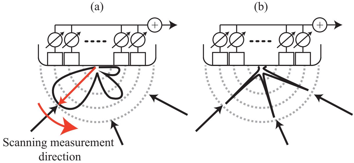
Figure 1.17: Schematic illustration of the Capon method. (a) Interference suppression using optimized weighting vector. (b) Estimated spectrum.
