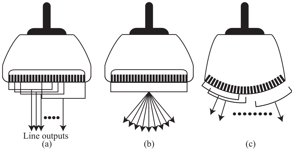
Figure 1.1: Probe types and scanning methods: (a) linear array probe with line scanning method, (b) linear array probe with a sector scanning method, and (c) convex array probe with a off-set sector scanning method.
