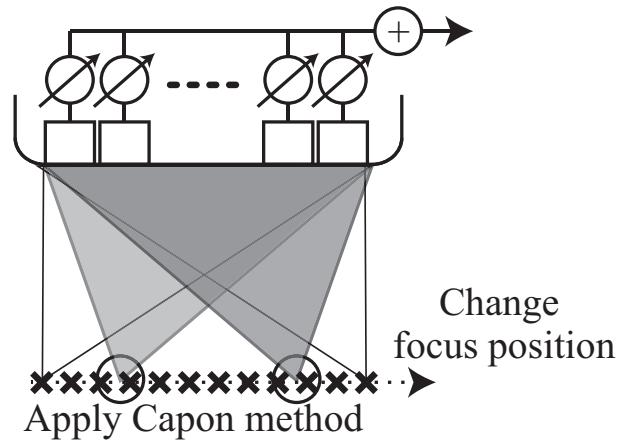
Figure 1.19: Schematic illustration of the Capon method for wide-band signals.
