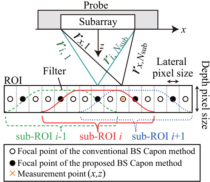
Figure 2.2: Schematic illustration of proposed method.(Reproduction from Okumura et al. (2016); Copyright(2016) The Japan Society of Applied Physics.)
