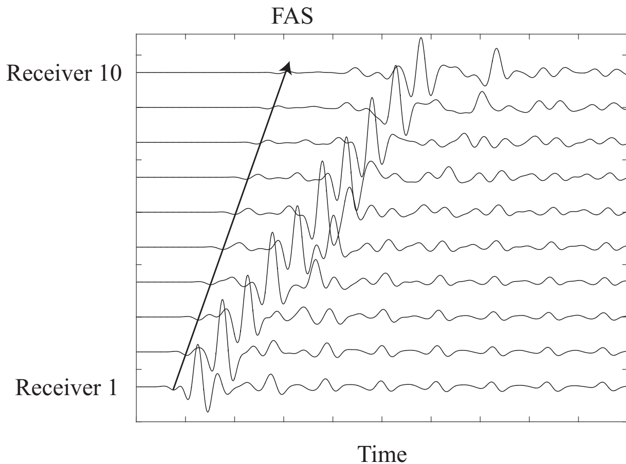
Figure 1.10: Guided waves and first arriving signals.
