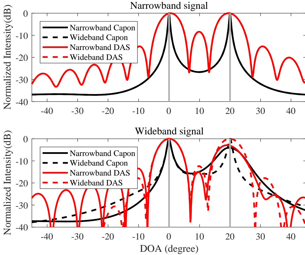
Figure 1.20: Performance dependences of beamforming techniques on the received signal bandwidth. The fractional bandwidths of the narrow and wide band signals are 1% and 50%, respectively.
